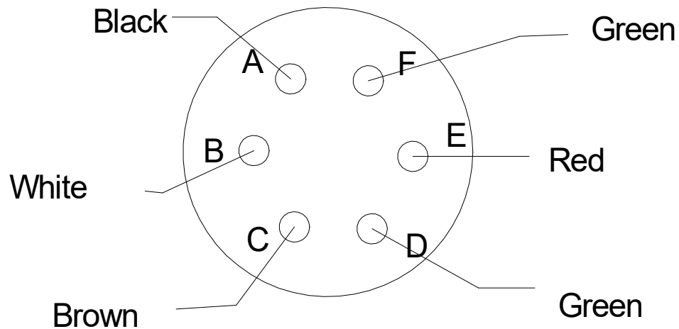
AAMI Connector From solder side of Male Connector
